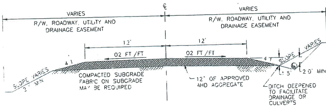
SUPPLEMENTAL SD-1B PRIVATELY MAINTAINED GRAVEL ROAD SECTION N T S
